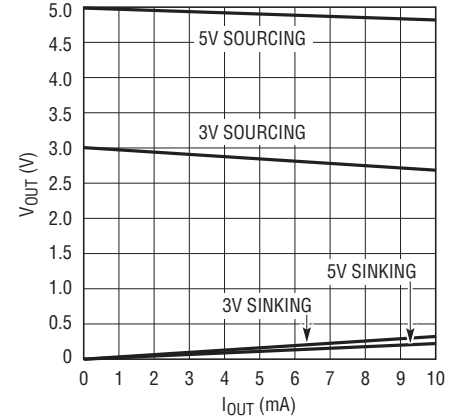
Headroom at Rails vs Output Current
